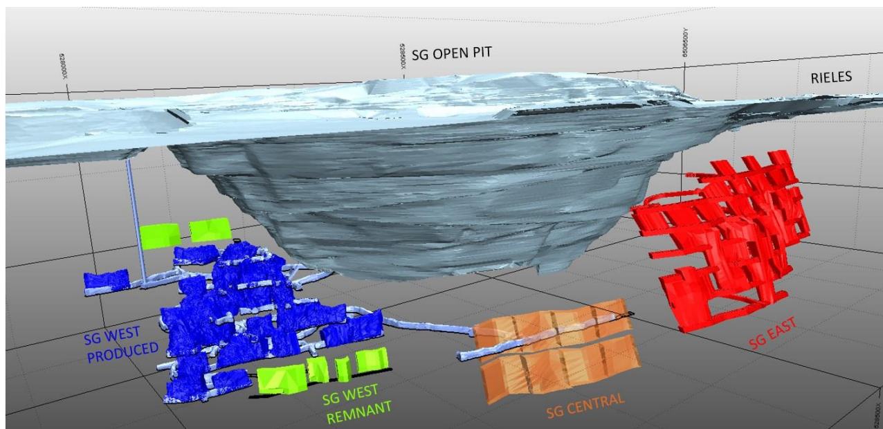
Isometric view of San Gregorio Pit & SG UG deposits at the end of Q3 18, including tunnel & development to SGC. Not to scale.
